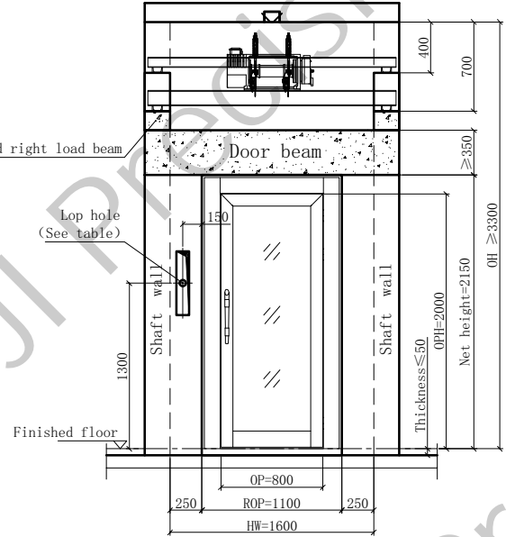
E direction Doorway schematic Facing Hoistway
