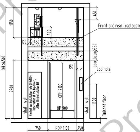
E/reserved hole/1: 60
