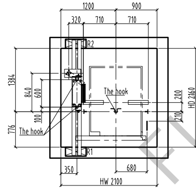
Overhead plan/1:60
