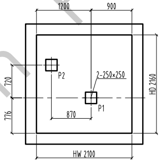
Pit plan/1: 60
