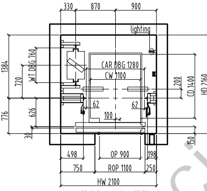
Hoistway plan/1:60
