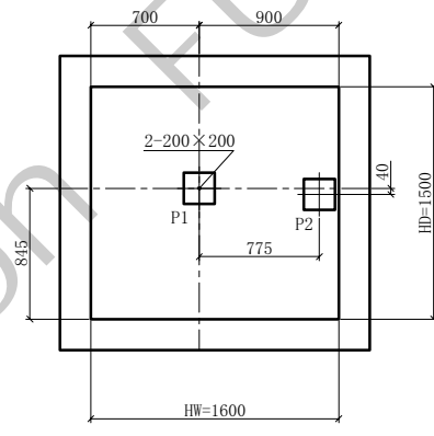
Pit plan
