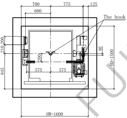
Overhead plan
